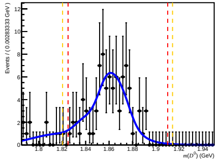
Passed DiF (after RICH1) ( 200 < nTracks < 600 , 3.6 < \eta < 5.0 , 3000 < p < 6000 )
