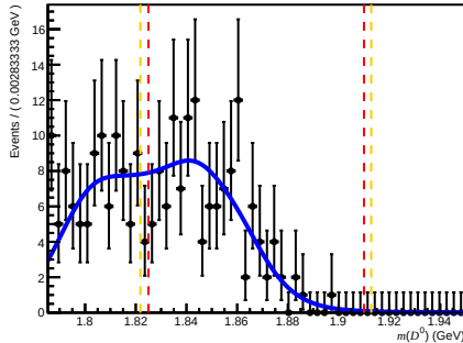
Passed DiF (before RICH1) ( 200 < nTracks < 600 , 3.6 < \eta < 5.0 , 15600 < p < 27000 )
