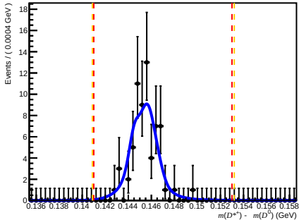
Passed DiF (before RICH1) ( 200 < n\text{Tracks} < 600 , 3.6 < \eta < 5.0 , 60000 < p < 100000 )
