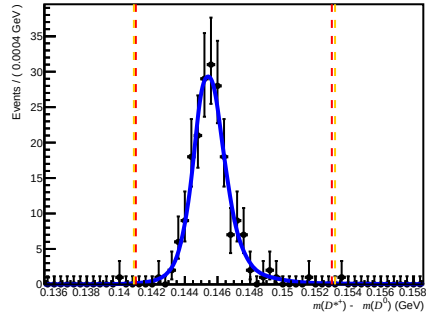
Failed DiF ( 200 < n\text{Tracks} < 600 , 3.6 < \eta < 5.0 , 60000 < p < 100000 )
