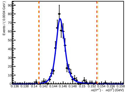
Passed DiF (after RICH1) ( 200 < n\text{Tracks} < 600 , 3.6 < \eta < 5.0 , 60000 < p < 100000 )
