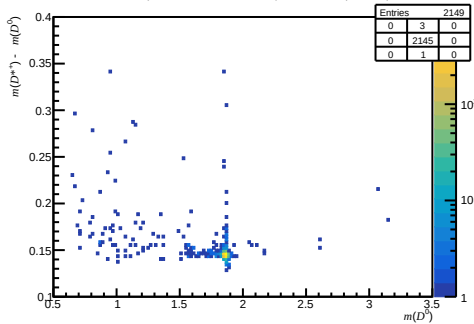
Failed DIF ( 0 < nTracks < 200 , 3.6 < \eta < 5.0 , 3000 < p < 6000 )
