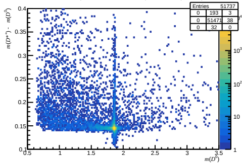
Failed non-DIF ( 0 < nTracks < 200 , 3.6 < \eta < 5.0 , 3000 < p < 6000 )
