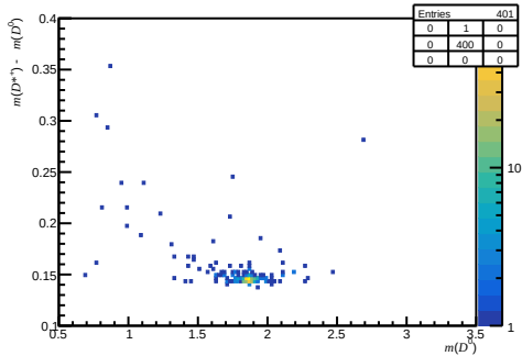
Passed DIF - after RICH1 ( 0 < nTracks < 200 , 3.6 < \eta < 5.0 , 3000 < p < 6000 )
