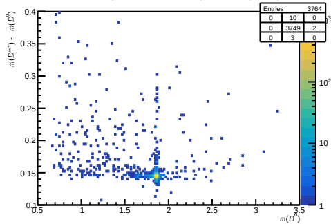
Passed non-DIF ( 0 < nTracks < 200 , 3.6 < \eta < 5.0 , 3000 < p < 6000 )
