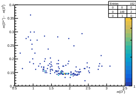
Passed DIF - before RICH1 ( 0 < nTracks < 200 , 3.6 < \eta < 5.0 , 3000 < p < 6000 )
