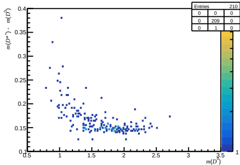
Passed DIF - before RICH1 ( 0 < n_{\text{Tracks}} < 200 , 3.6 < \eta < 5.0 , 6000 < p < 10000 )
