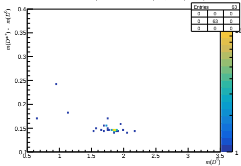
Passed DiF - before RICH1 (200 < nTracks < 600, 1.7 < \eta < 3.6, 10000 < p < 15600)
