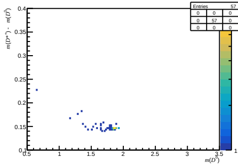
Passed DiF - before RICH1 (200 < nTracks < 600, 3.6 < \eta < 5.0, 27000 < p < 60000)
