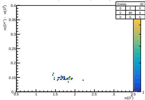
Passed DiF - before RICH1 ( 0 < n_{\text{Tracks}} < 200 , 3.6 < \eta < 5.0 , 60000 < p < 100000 )
