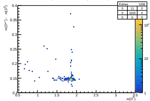
Passed non-DiF ( 0 < n_{\text{Tracks}} < 200 , 3.6 < \eta < 5.0 , 60000 < p < 100000 )
