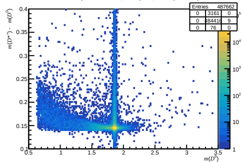
Failed non-DiF ( 0 < n_{\text{Tracks}} < 200 , 3.6 < \eta < 5.0 , 60000 < p < 100000 )
