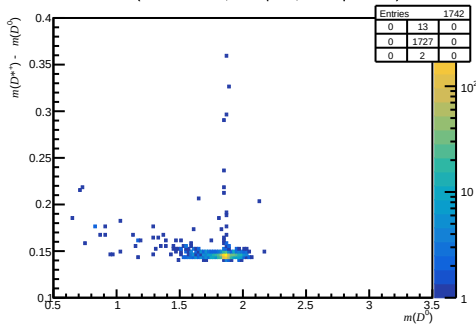
Failed DiF ( 0 < n_{\text{Tracks}} < 200 , 3.6 < \eta < 5.0 , 60000 < p < 100000 )
