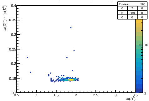
Passed DiF - after RICH1 ( 0 < n_{\text{Tracks}} < 200 , 3.6 < \eta < 5.0 , 60000 < p < 100000 )
