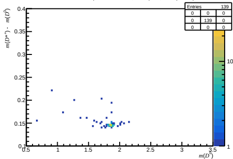
Passed DiF - after RICH1 (200 < nTracks < 600, 1.7 < \eta < 3.6, 3000 < p < 6000)
