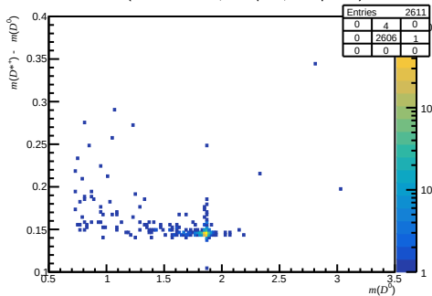
Failed DiF (200 < nTracks < 600, 1.7 < \eta < 3.6, 3000 < p < 6000)
