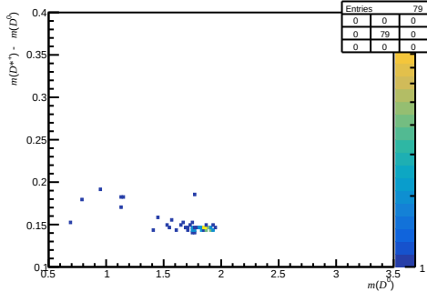
Passed DiF - after RICH1 (200 < nTracks < 600, 3.6 < \eta < 5.0, 10000 < p < 15600)
