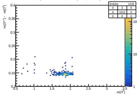
Failed DiF ( 0 < n_{\text{Tracks}} < 200 , 1.7 < \eta < 3.6 , 60000 < p < 100000 )
