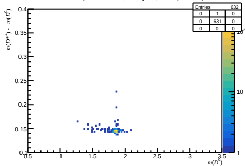
Passed non-DiF ( 0 < n_{\text{Tracks}} < 200 , 1.7 < \eta < 3.6 , 60000 < p < 100000 )
