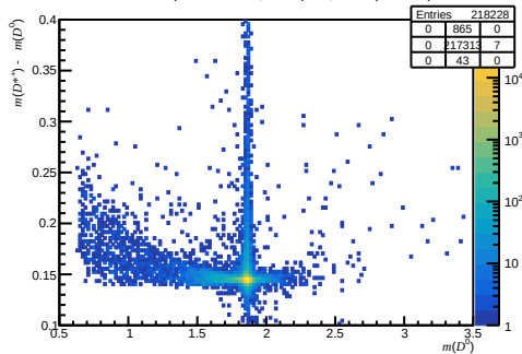
Failed non-DiF ( 0 < n_{\text{Tracks}} < 200 , 1.7 < \eta < 3.6 , 60000 < p < 100000 )
