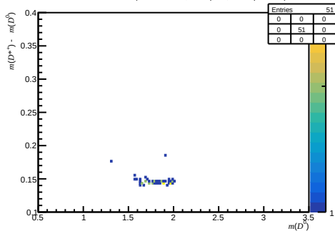
Passed DiF - before RICH1 ( 0 < n_{\text{Tracks}} < 200 , 1.7 < \eta < 3.6 , 60000 < p < 100000 )
