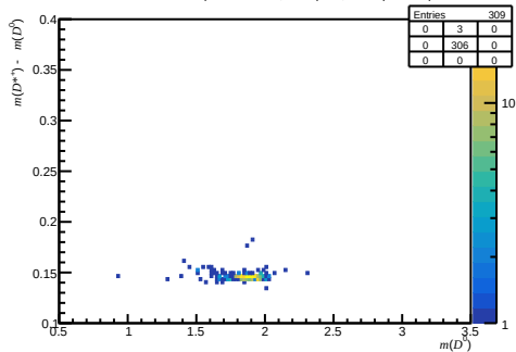
Passed DiF - after RICH1 ( 0 < n_{\text{Tracks}} < 200 , 1.7 < \eta < 3.6 , 60000 < p < 100000 )
