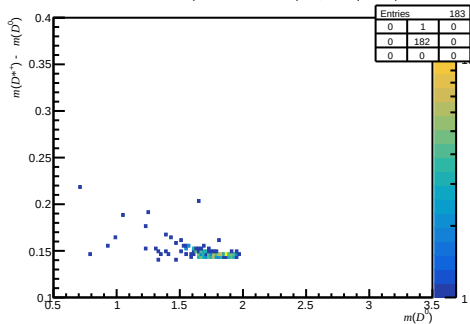
Passed DiF - before RICH1 ( 0 < n_{\text{Tracks}} < 200 , 3.6 < \eta < 5.0 , 27000 < p < 60000 )
