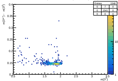
Passed DiF - after RICH1 ( 0 < n_{\text{Tracks}} < 200 , 3.6 < \eta < 5.0 , 27000 < p < 60000 )
