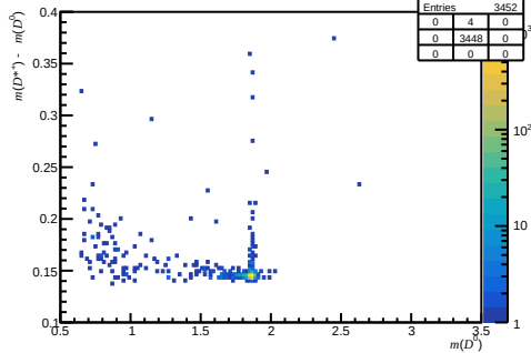
Passed non-DiF (200 < nTracks < 600, 1.7 < \eta < 3.6, 10000 < p < 15600)
