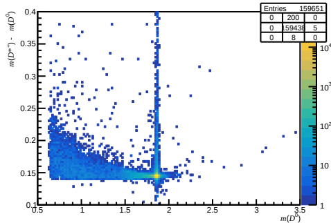
Failed non-DiF (200 < nTracks < 600, 1.7 < \eta < 3.6, 10000 < p < 15600)
