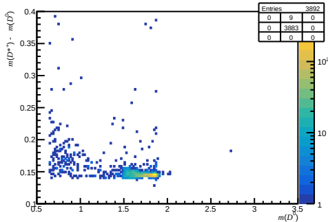
Passed DiF - after RICH1 ( 0 < nTracks < 200 , 1.7 < \eta < 3.6 , 3000 < p < 6000 )
