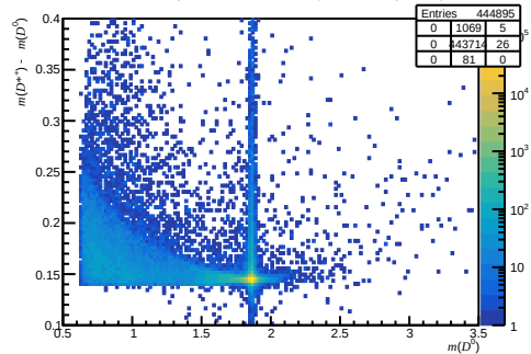
Failed non-DiF ( 0 < nTracks < 200 , 1.7 < \eta < 3.6 , 3000 < p < 6000 )
