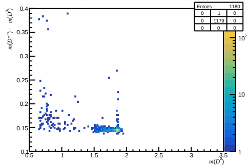
Passed non-DiF ( 0 < nTracks < 200 , 1.7 < \eta < 3.6 , 3000 < p < 6000 )
