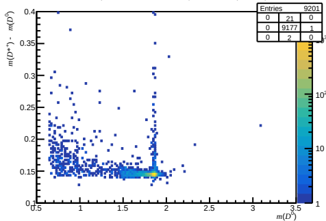
Failed DiF ( 0 < nTracks < 200 , 1.7 < \eta < 3.6 , 3000 < p < 6000 )
