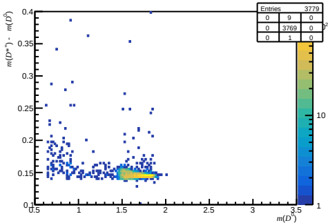
Passed DiF - before RICH1 ( 0 < nTracks < 200 , 1.7 < \eta < 3.6 , 3000 < p < 6000 )
