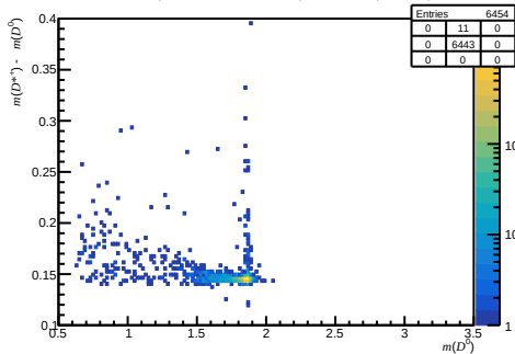
Failed DIF ( 0 < n_{\text{Tracks}} < 200 , 1.7 < \eta < 3.6 , 6000 < p < 10000 )
