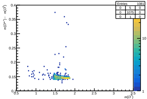
Passed DiF - before RICH1 ( 0 < nTracks < 200 , 3.6 < \eta < 5.0 , 15600 < p < 27000 )
