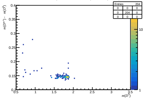
Passed DiF - after RICH1 (200 < nTracks < 600, 3.6 < \eta < 5.0, 6000 < p < 10000)
