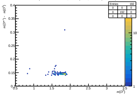
Failed DiF (200 < nTracks < 600, 3.6 < \eta < 5.0, 15600 < p < 27000)
