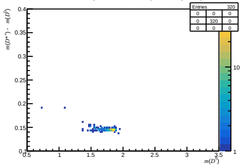
Passed DiF - after RICH1 (200 < nTracks < 600, 3.6 < \eta < 5.0, 15600 < p < 27000)
