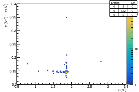
Passed non-DiF (200 < nTracks < 600, 3.6 < \eta < 5.0, 27000 < p < 60000)
