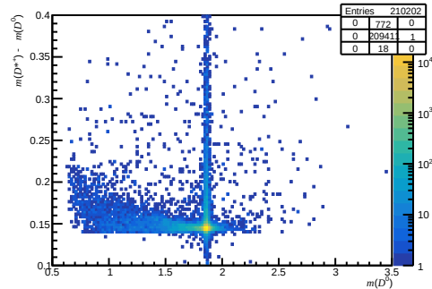
Failed non-DiF (200 < nTracks < 600, 3.6 < \eta < 5.0, 27000 < p < 60000)
