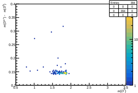
Passed DiF - after RICH1 (200 < nTracks < 600, 3.6 < \eta < 5.0, 27000 < p < 60000)
