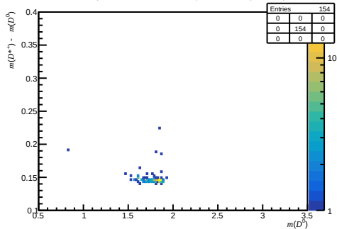
Failed DiF (200 < nTracks < 600, 3.6 < \eta < 5.0, 27000 < p < 60000)
