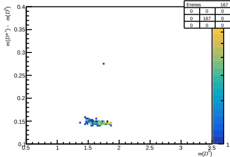
Passed DiF - before RICH1 (200 < nTracks < 600, 3.6 < \eta < 5.0, 27000 < p < 60000)
