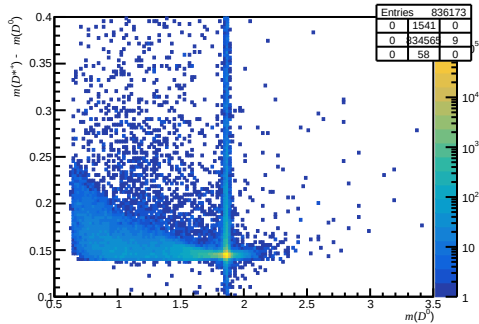
Failed non-DiF ( 0 < n_{\text{Tracks}} < 200 , 1.7 < \eta < 3.6 , 10000 < p < 15600 )
