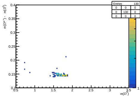
Passed DiF - before RICH1 ( 0 < n_{\text{Tracks}} < 200 , 1.7 < \eta < 3.6 , 10000 < p < 15600 )
