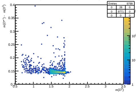
Failed DiF ( 0 < n_{\text{Tracks}} < 200 , 1.7 < \eta < 3.6 , 10000 < p < 15600 )
