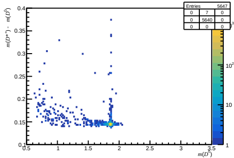
Passed non-DiF ( 0 < n_{\text{Tracks}} < 200 , 1.7 < \eta < 3.6 , 10000 < p < 15600 )
