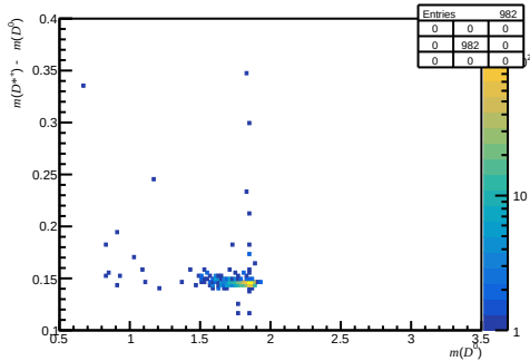
Passed DiF - after RICH1 ( 0 < n_{\text{Tracks}} < 200 , 1.7 < \eta < 3.6 , 10000 < p < 15600 )
