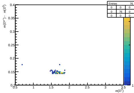
Passed DiF - before RICH1 ( 0 < n_{\text{Tracks}} < 200 , 1.7 < \eta < 3.6 , 15600 < p < 27000 )
