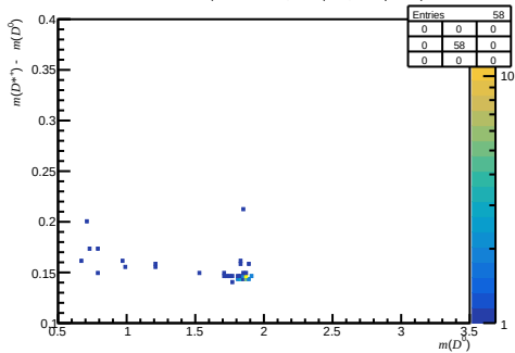
Passed DiF - after RICH1 ( 0 < n_{\text{Tracks}} < 200 , 3.6 < \eta < 5.0 , 3000 < p < 6000 )
