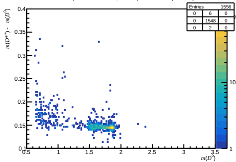
Failed DiF ( 0 < n_{\text{Tracks}} < 200 , 3.6 < \eta < 5.0 , 3000 < p < 6000 )
