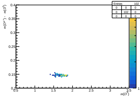
Passed DiF - before RICH1 (200 < nTracks < 600, 1.7 < \eta < 3.6, 6000 < p < 10000)
