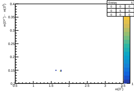
Passed DiF - before RICH1 (200 < nTracks < 600, 3.6 < \eta < 5.0, 60000 < p < 100000)
