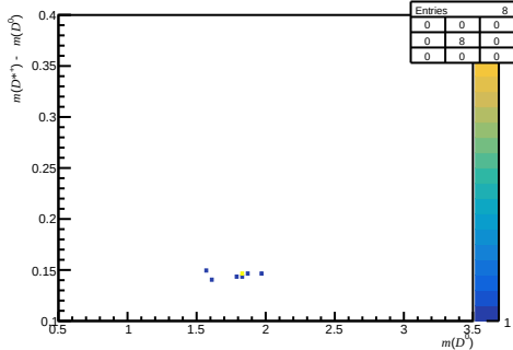
Passed DiF - after RICH1 (200 < nTracks < 600, 3.6 < \eta < 5.0, 60000 < p < 100000)
