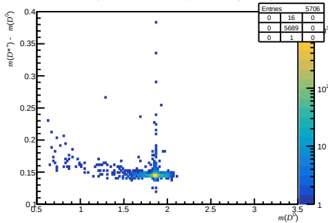
Failed DiF ( 0 < n_{\text{Tracks}} < 200 , 1.7 < \eta < 3.6 , 27000 < p < 60000 )
