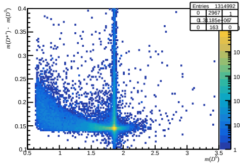
Failed non-DiF ( 0 < n_{\text{Tracks}} < 200 , 1.7 < \eta < 3.6 , 27000 < p < 60000 )
