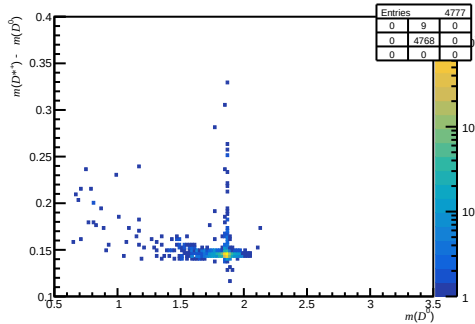
Passed non-DiF ( 0 < n_{\text{Tracks}} < 200 , 1.7 < \eta < 3.6 , 27000 < p < 60000 )
