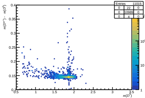
Passed DiF - after RICH1 ( 0 < n_{\text{Tracks}} < 200 , 1.7 < \eta < 3.6 , 27000 < p < 60000 )
