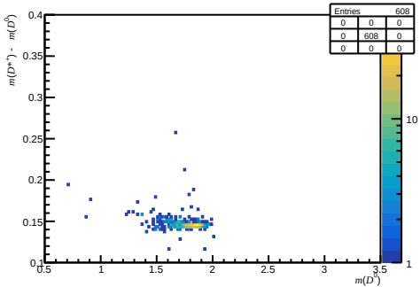
Passed DiF - before RICH1 ( 0 < n_{\text{Tracks}} < 200 , 1.7 < \eta < 3.6 , 27000 < p < 60000 )
