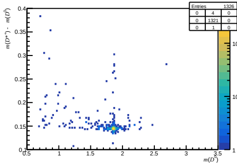
Passed DIF - after RICH1 ( 0 < nTracks < 200 , 3.6 < \eta < 5.0 , 3000 < p < 6000 )
