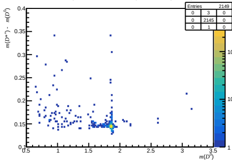
Failed DIF ( 0 < nTracks < 200 , 3.6 < \eta < 5.0 , 3000 < p < 6000 )
