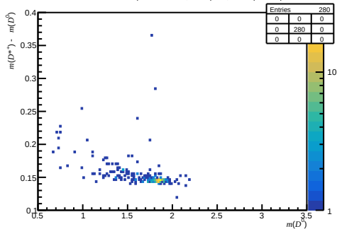
Passed DiF - before RICH1 ( 0 < n_{\text{Tracks}} < 200 , 3.6 < \eta < 5.0 , 15600 < p < 27000 )
