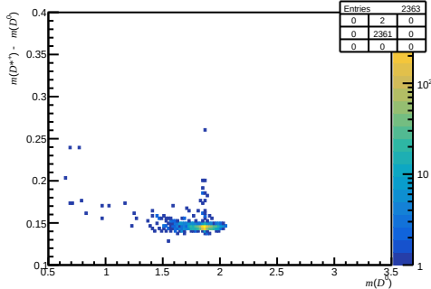
Passed DiF - after RICH1 (200 < nTracks < 600, 1.7 < \eta < 3.6, 27000 < p < 60000)
