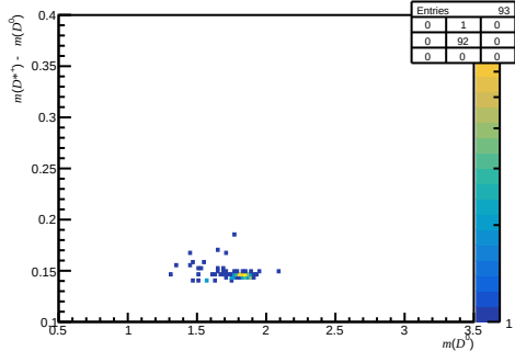
Passed DiF - before RICH1 (200 < nTracks < 600, 1.7 < \eta < 3.6, 27000 < p < 60000)
