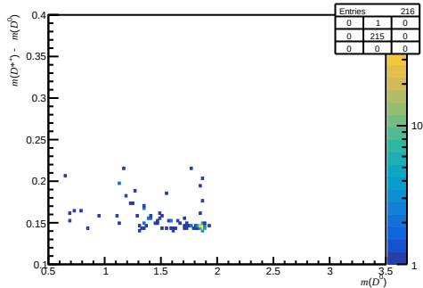
Passed non-DiF ( 0 < n_{\text{Tracks}} < 200 , 3.6 < \eta < 5.0 , 15600 < p < 27000 )
