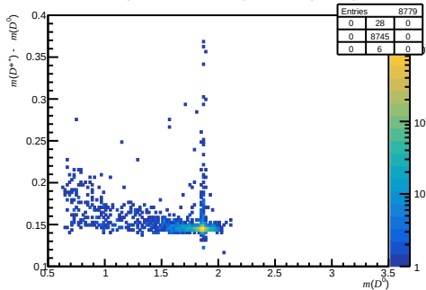
Failed DiF ( 0 < n_{\text{Tracks}} < 200 , 3.6 < \eta < 5.0 , 15600 < p < 27000 )
