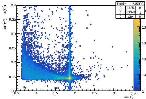
Failed non-DiF ( 0 < n_{\text{Tracks}} < 200 , 3.6 < \eta < 5.0 , 15600 < p < 27000 )
