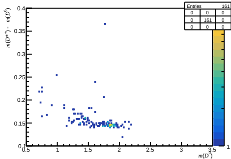
Passed DiF - before RICH1 ( 0 < n_{\text{Tracks}} < 200 , 3.6 < \eta < 5.0 , 15600 < p < 27000 )
