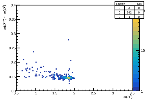
Passed DiF - after RICH1 ( 0 < n_{\text{Tracks}} < 200 , 3.6 < \eta < 5.0 , 15600 < p < 27000 )
