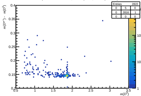
Failed DiF (200 < nTracks < 600, 1.7 < \eta < 3.6, 3000 < p < 6000)
