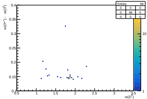
Passed non-DiF (200 < nTracks < 600, 1.7 < \eta < 3.6, 3000 < p < 6000)
