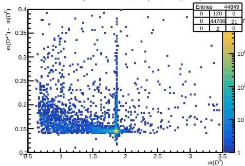
Failed non-DiF (200 < nTracks < 600, 1.7 < \eta < 3.6, 3000 < p < 6000)
