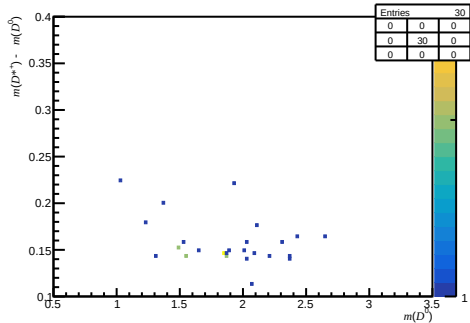
Passed DiF - before RICH1 (200 < nTracks < 600, 1.7 < \eta < 3.6, 3000 < p < 6000)
