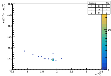
Passed DiF - after RICH1 (200 < nTracks < 600, 1.7 < \eta < 3.6, 3000 < p < 6000)
