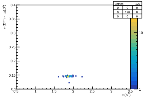
Passed DiF - after RICH1 (200 < nTracks < 600, 1.7 < \eta < 3.6, 60000 < p < 100000)
