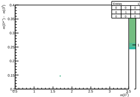
Passed DiF - before RICH1 (200 < nTracks < 600, 1.7 < \eta < 3.6, 60000 < p < 100000)
