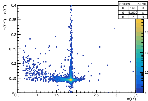
Failed non-DiF (200 < nTracks < 600, 1.7 < \eta < 3.6, 60000 < p < 100000)
