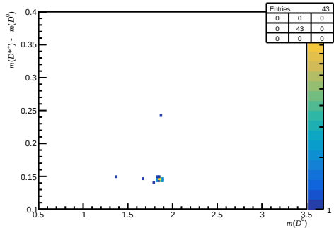
Passed non-DiF (200 < nTracks < 600, 1.7 < \eta < 3.6, 60000 < p < 100000)
