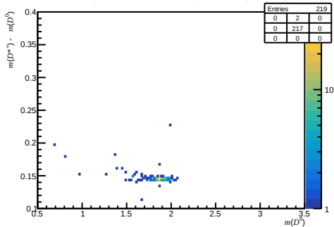
Failed DiF (200 < nTracks < 600, 1.7 < \eta < 3.6, 60000 < p < 100000)
