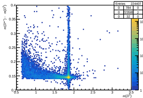
Failed non-DiF (200 < nTracks < 600, 3.6 < \eta < 5.0, 27000 < p < 60000)
