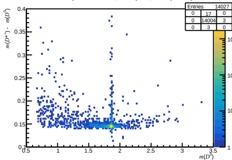
Failed DiF ( 0 < n_{\text{Tracks}} < 200 , 1.7 < \eta < 3.6 , 3000 < p < 6000 )
