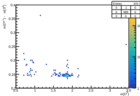
Passed DiF - after RICH1 ( 0 < n_{\text{Tracks}} < 200 , 1.7 < \eta < 3.6 , 3000 < p < 6000 )
