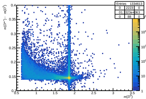
Failed non-DiF ( 0 < nTracks < 200 , 1.7 < \eta < 3.6 , 15600 < p < 27000 )
