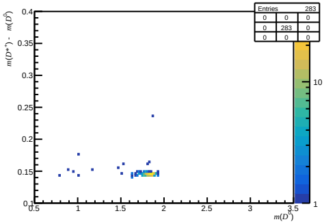
Passed DiF - before RICH1 ( 0 < nTracks < 200 , 1.7 < \eta < 3.6 , 15600 < p < 27000 )
