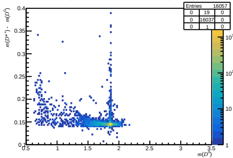
Failed DiF ( 0 < nTracks < 200 , 1.7 < \eta < 3.6 , 15600 < p < 27000 )
