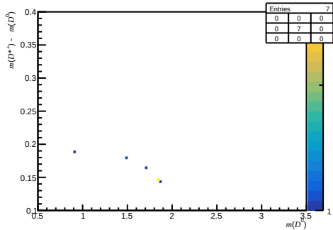
Passed DiF - before RICH1 ( 0 < n_{\text{Tracks}} < 200 , 3.6 < \eta < 5.0 , 3000 < p < 6000 )
