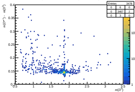
Failed DiF ( 0 < n_{\text{Tracks}} < 200 , 3.6 < \eta < 5.0 , 3000 < p < 6000 )
