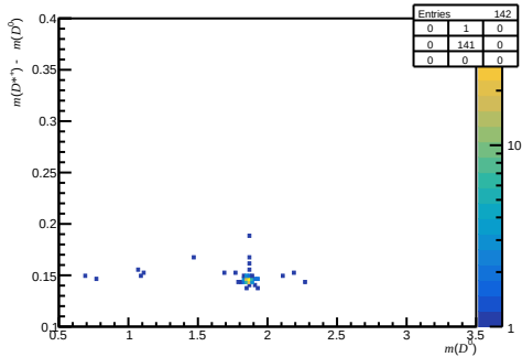
Passed DiF - after RICH1 ( 0 < n_{\text{Tracks}} < 200 , 3.6 < \eta < 5.0 , 3000 < p < 6000 )
