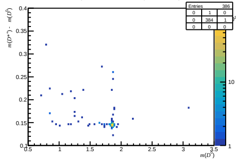
Passed non-DiF ( 0 < n_{\text{Tracks}} < 200 , 3.6 < \eta < 5.0 , 3000 < p < 6000 )
