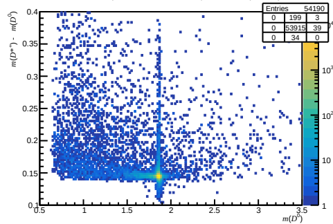
Failed non-DiF ( 0 < n_{\text{Tracks}} < 200 , 3.6 < \eta < 5.0 , 3000 < p < 6000 )
