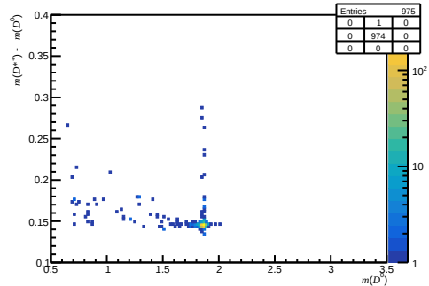
Passed non-DiF ( 0 < nTracks < 200 , 3.6 < \eta < 5.0 , 15600 < p < 27000 )
