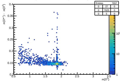
Failed DiF ( 0 < nTracks < 200 , 3.6 < \eta < 5.0 , 15600 < p < 27000 )
