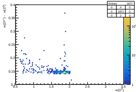
Passed DiF - after RICH1 ( 0 < nTracks < 200 , 3.6 < \eta < 5.0 , 15600 < p < 27000 )
