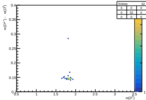
Passed DiF - before RICH1 ( 0 < nTracks < 200 , 3.6 < \eta < 5.0 , 15600 < p < 27000 )
