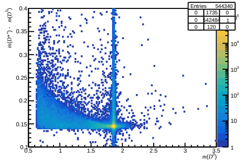
Failed non-DiF ( 0 < nTracks < 200 , 3.6 < \eta < 5.0 , 15600 < p < 27000 )
