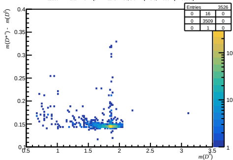
Passed DiF - after RICH1 ( 0 < n_{\text{Tracks}} < 200 , 3.6 < \eta < 5.0 , 27000 < p < 60000 )
