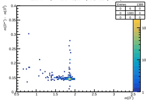
Passed non-DiF ( 0 < n_{\text{Tracks}} < 200 , 3.6 < \eta < 5.0 , 27000 < p < 60000 )
