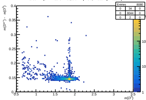
Failed DiF ( 0 < n_{\text{Tracks}} < 200 , 3.6 < \eta < 5.0 , 27000 < p < 60000 )
