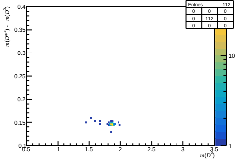
Passed DiF - after RICH1 (200 < nTracks < 600, 3.6 < \eta < 5.0, 6000 < p < 10000)
