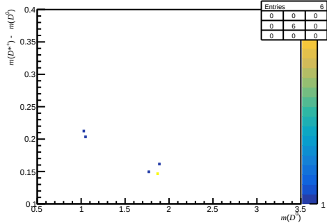
Passed DiF - before RICH1 (200 < nTracks < 600, 3.6 < \eta < 5.0, 6000 < p < 10000)
