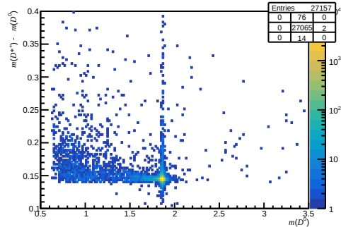
Failed non-DiF (200 < nTracks < 600, 3.6 < \eta < 5.0, 6000 < p < 10000)
