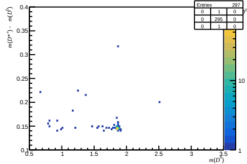
Passed non-DiF (200 < nTracks < 600, 3.6 < \eta < 5.0, 6000 < p < 10000)
