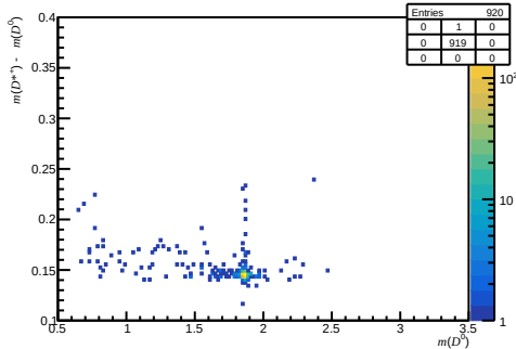
Failed DiF (200 < nTracks < 600, 3.6 < \eta < 5.0, 6000 < p < 10000)
