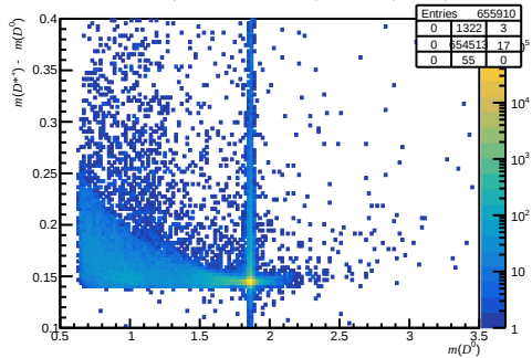
Failed non-DIF ( 0 < n_{\text{Tracks}} < 200 , 1.7 < \eta < 3.6 , 6000 < p < 10000 )
