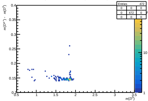
Failed DIF ( 0 < n_{\text{Tracks}} < 200 , 1.7 < \eta < 3.6 , 6000 < p < 10000 )
