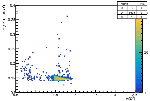
Passed DIF - before RICH1 ( 0 < n_{\text{Tracks}} < 200 , 1.7 < \eta < 3.6 , 6000 < p < 10000 )
