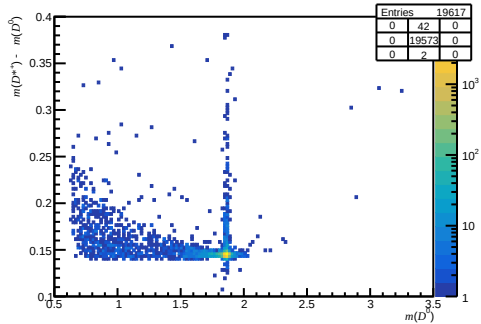
Passed non-DIF ( 0 < n_{\text{Tracks}} < 200 , 1.7 < \eta < 3.6 , 6000 < p < 10000 )
