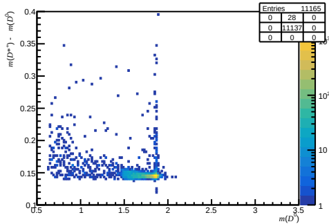
Passed DIF - after RICH1 ( 0 < n_{\text{Tracks}} < 200 , 1.7 < \eta < 3.6 , 6000 < p < 10000 )
