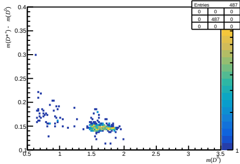
Passed DiF - before RICH1 ( 0 < n_{\text{Tracks}} < 200 , 3.6 < \eta < 5.0 , 3000 < p < 6000 )
