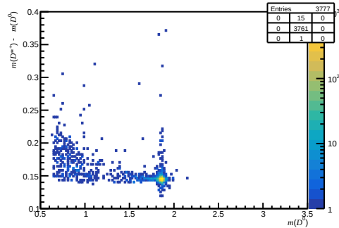
Passed non-DIF ( 0 < n_{\text{Tracks}} < 200 , 3.6 < \eta < 5.0 , 6000 < p < 10000 )
