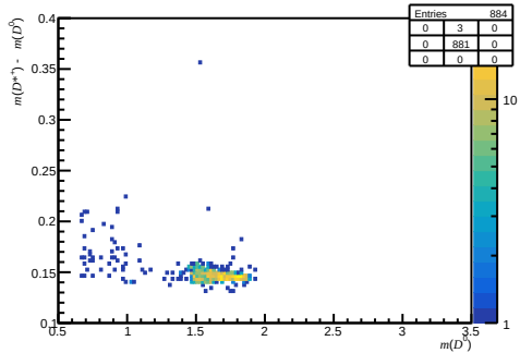
Passed DIF - before RICH1 ( 0 < n_{\text{Tracks}} < 200 , 3.6 < \eta < 5.0 , 6000 < p < 10000 )
