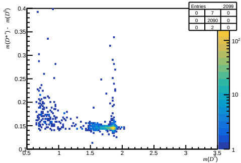
Passed DIF - after RICH1 ( 0 < n_{\text{Tracks}} < 200 , 3.6 < \eta < 5.0 , 6000 < p < 10000 )
