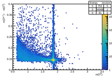
Failed non-DiF ( 0 < n_{\text{Tracks}} < 200 , 3.6 < \eta < 5.0 , 10000 < p < 15600 )
