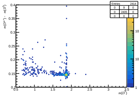
Passed non-DiF ( 0 < n_{\text{Tracks}} < 200 , 3.6 < \eta < 5.0 , 10000 < p < 15600 )
