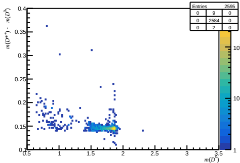
Passed DiF - after RICH1 ( 0 < n_{\text{Tracks}} < 200 , 3.6 < \eta < 5.0 , 10000 < p < 15600 )
