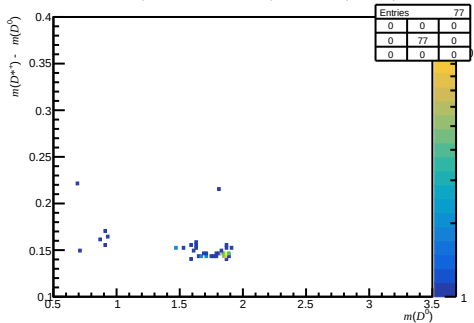
Failed DiF ( 0 < n_{\text{Tracks}} < 200 , 3.6 < \eta < 5.0 , 10000 < p < 15600 )
