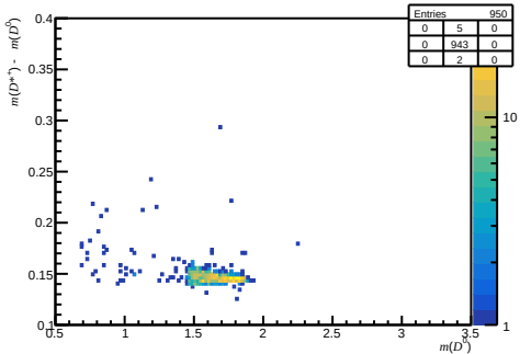
Passed DiF - before RICH1 ( 0 < n_{\text{Tracks}} < 200 , 3.6 < \eta < 5.0 , 10000 < p < 15600 )
