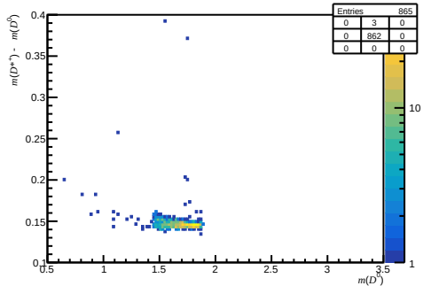
Passed DiF - before RICH1 ( 0 < n_{\text{Tracks}} < 200 , 3.6 < \eta < 5.0 , 27000 < p < 60000 )
