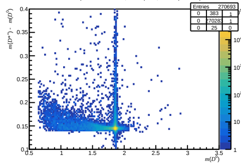
Failed non-DiF (200 < nTracks < 600, 1.7 < \eta < 3.6, 15600 < p < 27000)
