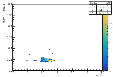
Passed DiF - before RICH1 (200 < nTracks < 600, 1.7 < \eta < 3.6, 15600 < p < 27000)
