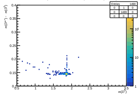
Passed non-DiF (200 < nTracks < 600, 1.7 < \eta < 3.6, 15600 < p < 27000)
