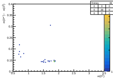
Passed non-DiF (200 < nTracks < 600, 1.7 < \eta < 3.6, 3000 < p < 6000)
