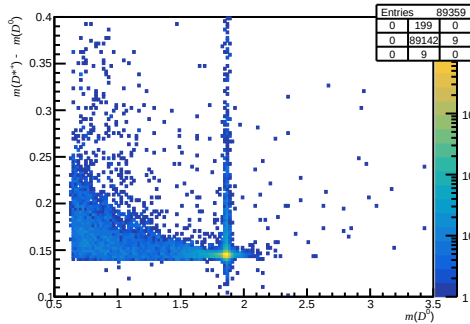
Failed non-DiF (200 < nTracks < 600, 1.7 < \eta < 3.6, 3000 < p < 6000)
