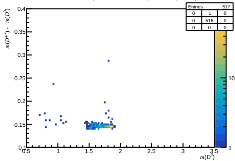
Passed DiF - after RICH1 (200 < nTracks < 600, 1.7 < \eta < 3.6, 6000 < p < 10000)
