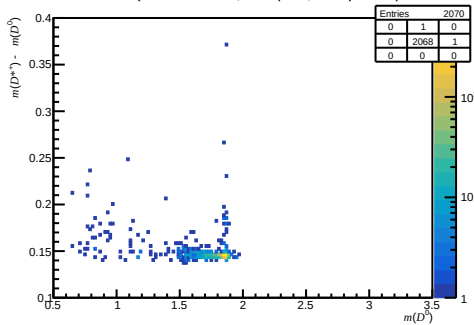
Failed DiF (200 < nTracks < 600, 1.7 < \eta < 3.6, 6000 < p < 10000)
