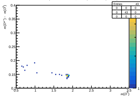
Passed non-DiF (200 < nTracks < 600, 3.6 < \eta < 5.0, 3000 < p < 6000)
