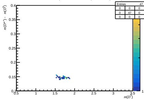
Passed DiF - before RICH1 ( 0 < n_{\text{Tracks}} < 200 , 1.7 < \eta < 3.6 , 27000 < p < 60000 )
