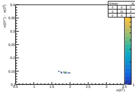
Passed non-DiF ( 0 < n_{\text{Tracks}} < 200 , 1.7 < \eta < 3.6 , 60000 < p < 100000 )
