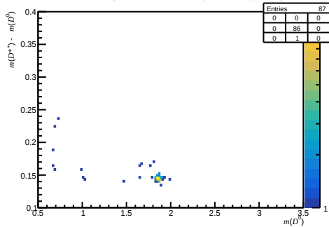
Passed non-DiF ( 0 < n_{\text{Tracks}} < 200 , 3.6 < \eta < 5.0 , 3000 < p < 6000 )
