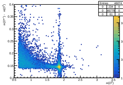
Failed non-DiF ( 0 < n_{\text{Tracks}} < 200 , 3.6 < \eta < 5.0 , 3000 < p < 6000 )
